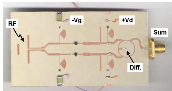
Fig. 4 Picture of low noise active integrated antenna receiver.
