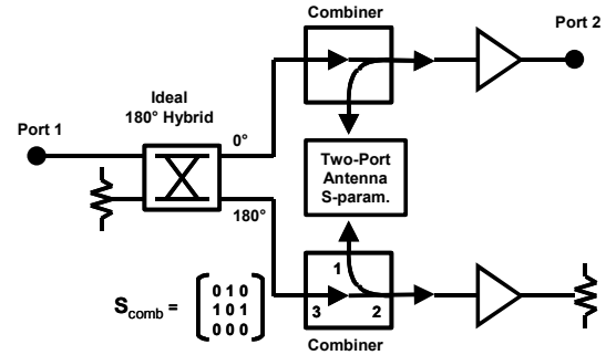
Fig. 3 Schematic of LNA design used for simulation purposes.
