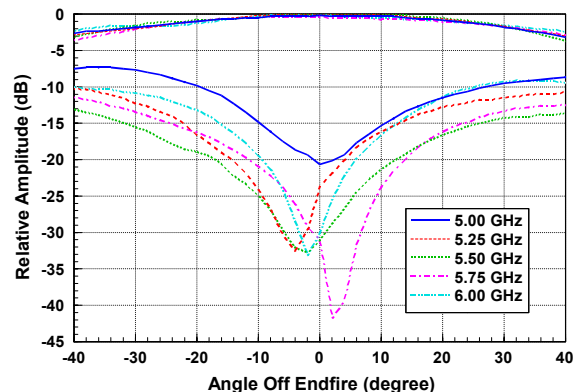
Fig.6 Sum and difference radiation patterns.
